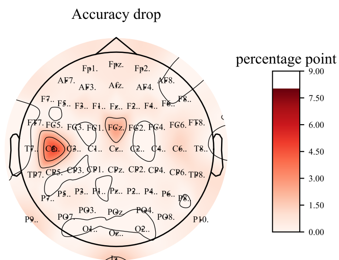
Fig. 3. The heat map of performance drop in accuracy of AADNet SI model on the KUL dataset when one channel is left out.
