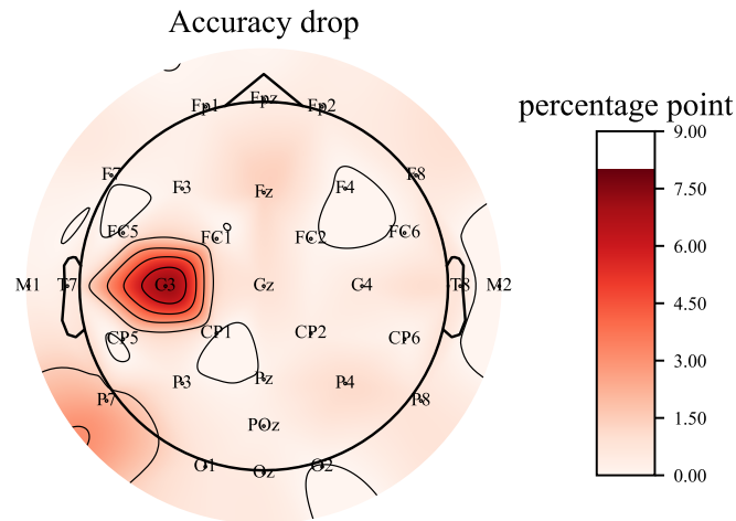
Fig. 1. The heat map of performance drop in accuracy of AADNet SI model on the EventAAD dataset when one channel is left out.
